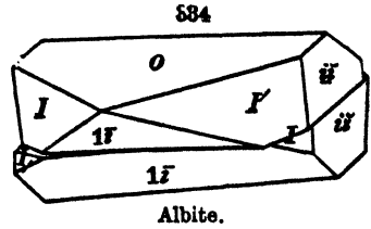
Albite.
